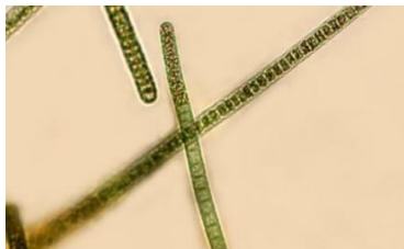
Oscillatoria sp.
