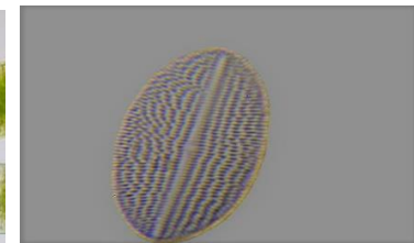
Cocconeis sp.
