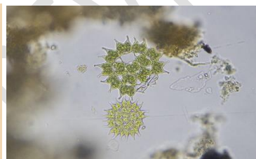
Pediastrum sp.
