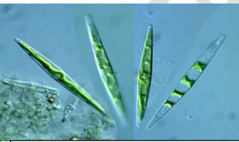
Closteriopsis sp.
