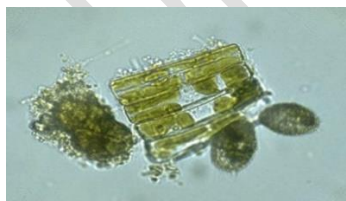
Diatoma sp.
