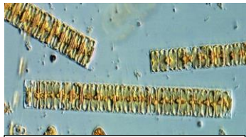
Achnanthes sp.
