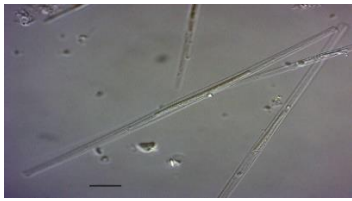
Fragilaria sp.
