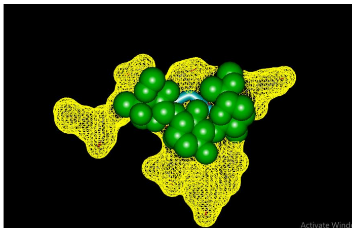
Fig.7. Complex form of Gentamicin (green color) with TP53 (yellow color) showing the electrostatic force of attraction using Discovery Studio software.
