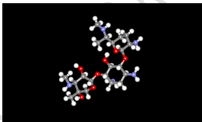
Fig.2. 3D structure of Gentamicin in ball and stick model viewed using Discovery Studio Software.
