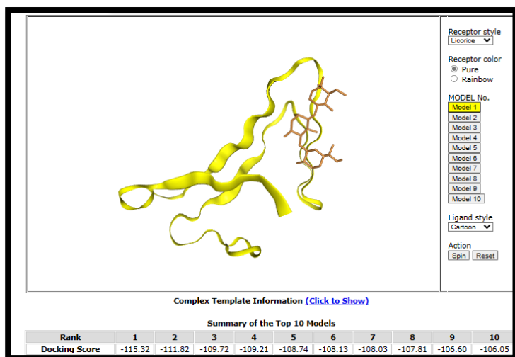
Fig.1. Complex form of Gentamicin with tumor protein, TP53 using H-Dock server showing the corresponding binding scores.
