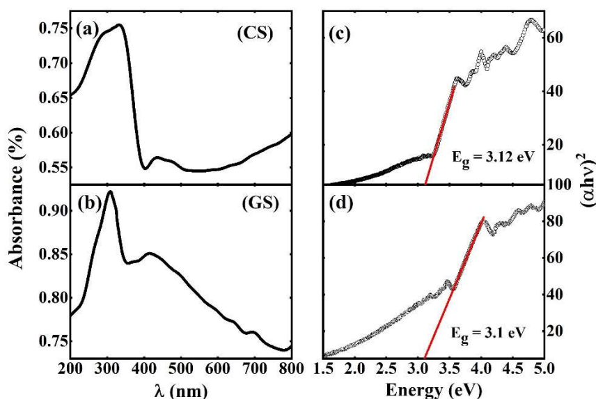
Fig. 5: UV-Vis absorbance spectra and Tauc plots of Ag/ZnO nanocomposite synthesized using co-precipitation and green synthesis method
