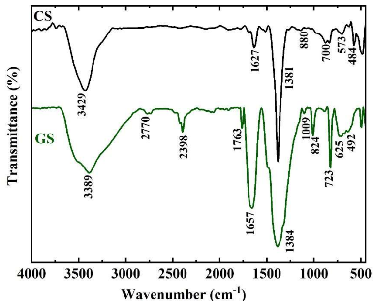
Fig. 3: FT-IR spectra of CS and GS samples
