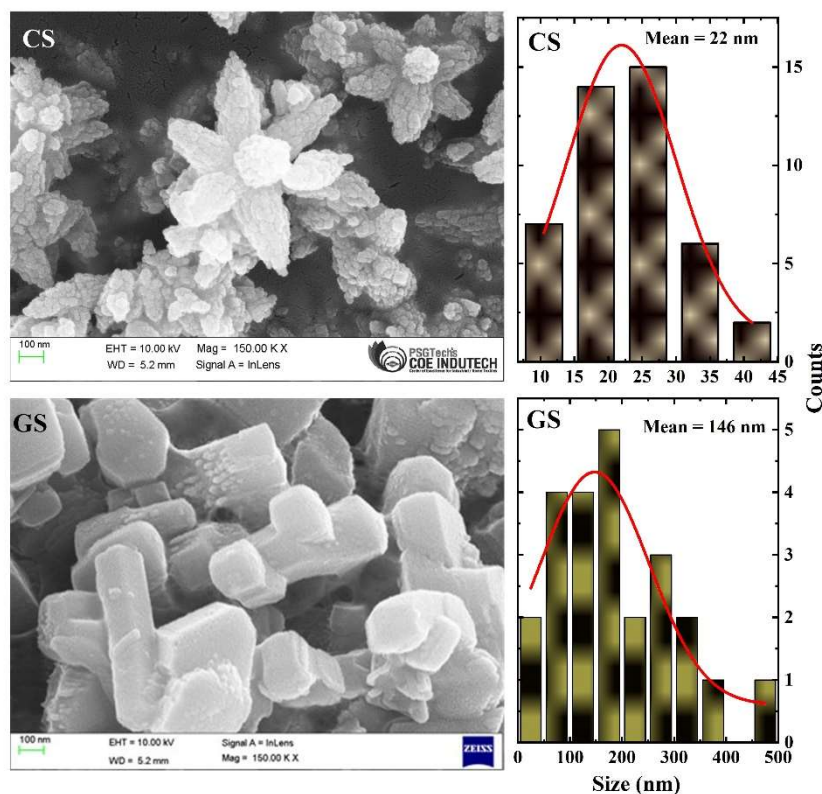
Fig. 4: FESEM morphological image of Ag/ZnO nanocomposite synthesized using co-precipitation method (Top) and green synthesis (Bottom)
