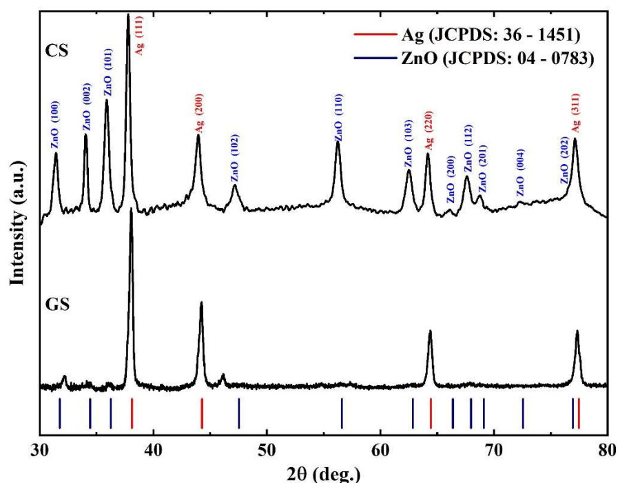
Fig. 2: Powder XRD patterns of Ag/ZnO nanocomposites synthesized through (Top) chemical (CS) and (Bottom) green synthesis (GS) methods
