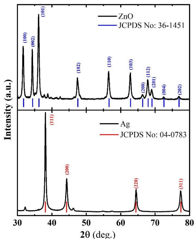
Fig. 1: Powder XRD pattern of pure ZnO (Top) and Ag (Bottom) nanoparticles synthesized using chemical method and compared with JCPDS card no: 36-1451 and 04-0783 respectively
